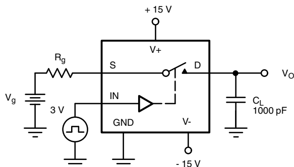
Figure 5. Charge Injection
