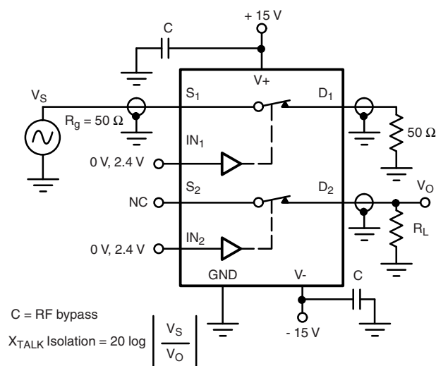
Figure 4. Channel-to-Channel Crosstalk
