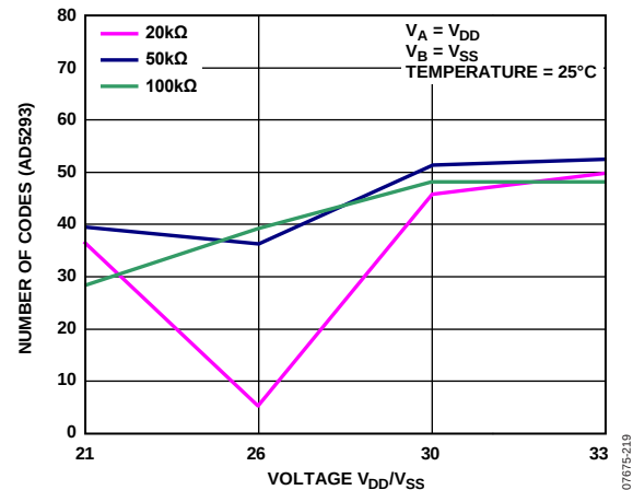
Figure 38. Code Range > 1% R-Tolerance Error vs. Voltage
