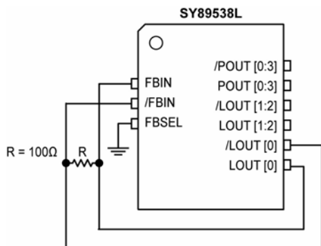
Figure 3a. Zero Delay Mode (LVDS Output)
