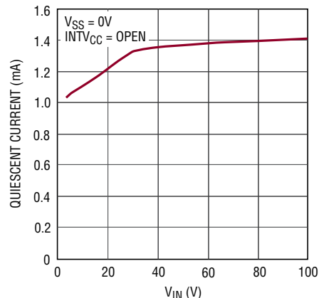
Quiescent Current vs V_{IN} Voltage
