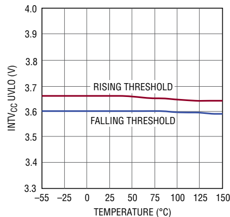
INTV_{CC} Undervoltage Lockout vs Temperature
