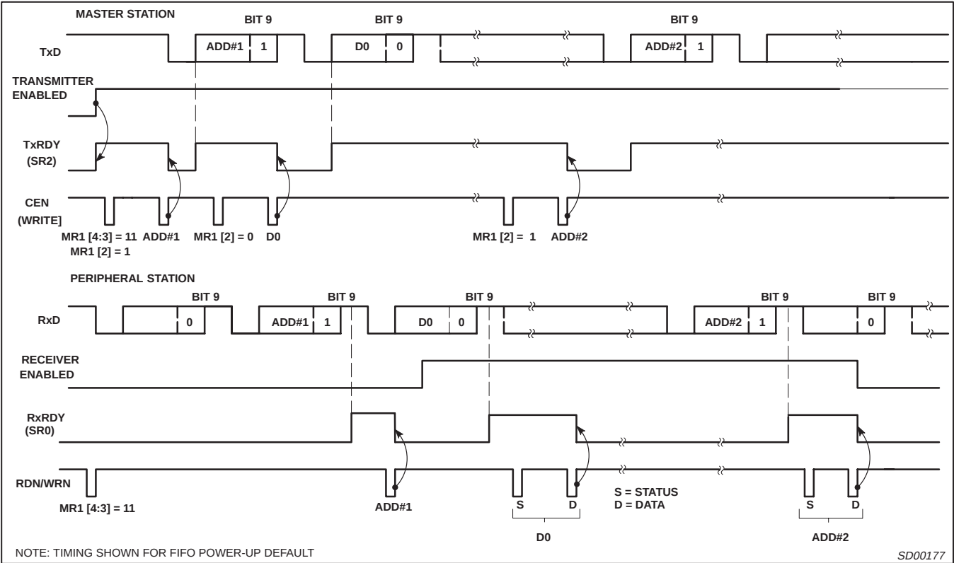
Figure 18. Wake-Up Mode
