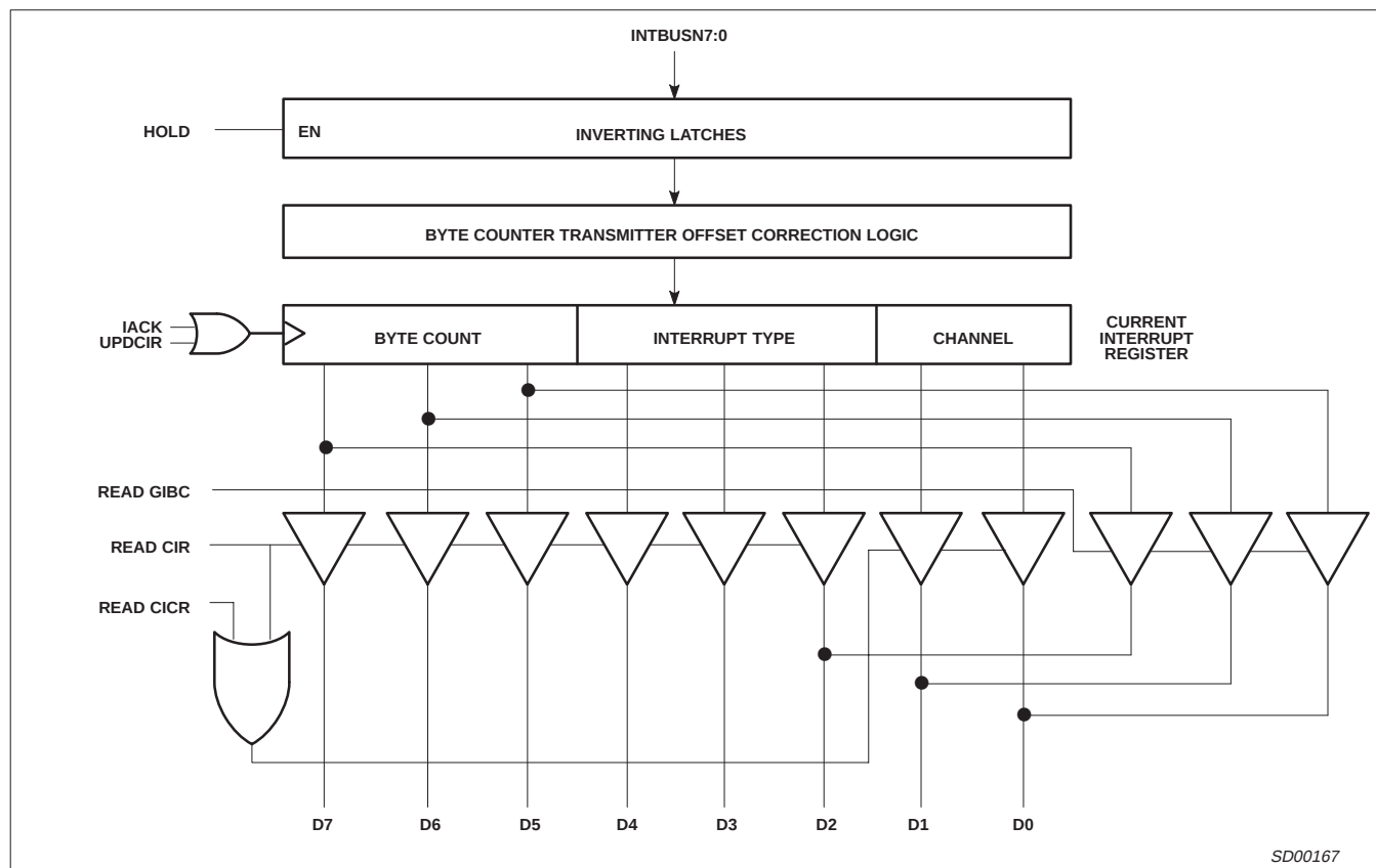
Figure 8. Current Interrupt Register Logic
