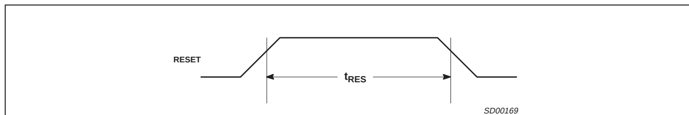
Figure 10. Reset Timing
