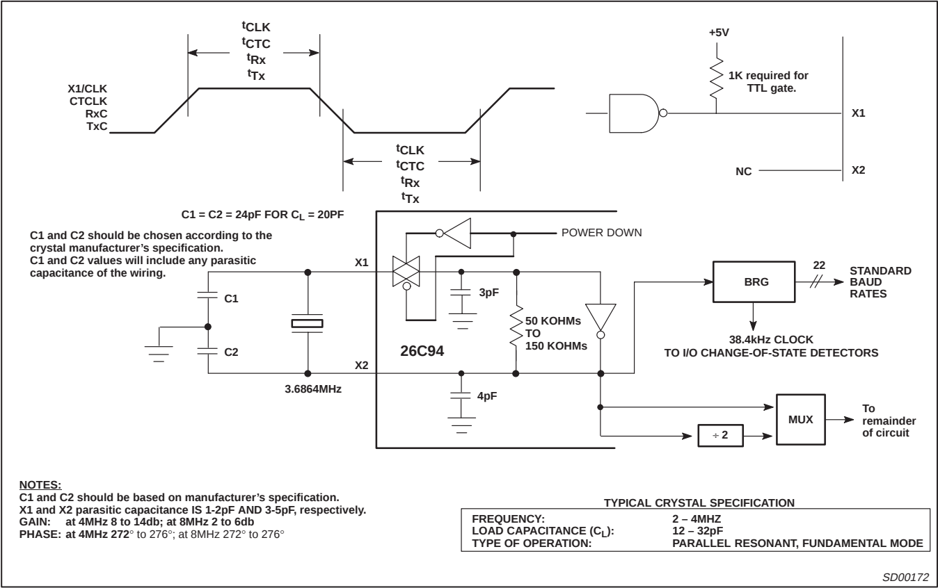
Figure 13. Clock Timing
