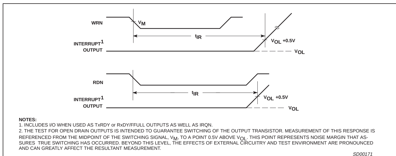
Figure 12. Interrupt Timing
