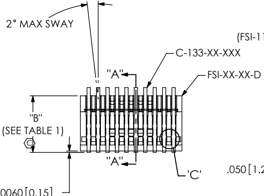
FIG 1 (FSI-110-06-XXX-D SHOWN)
