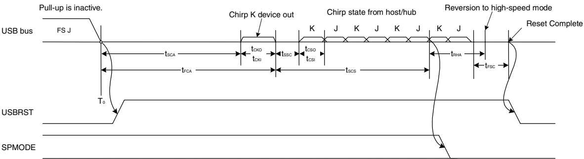
Figure 2-17. USB Reset from Suspend State (2)
