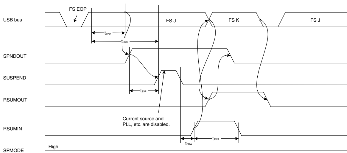
Figure 2-20. Remote Wakeup on USB 1.1
