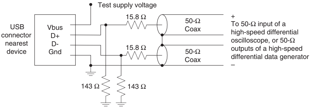
Figure 2-5. Receiver Measurement Fixtures
