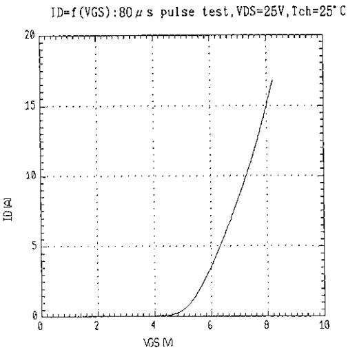
伝達特性 Typical transfer characteristic
