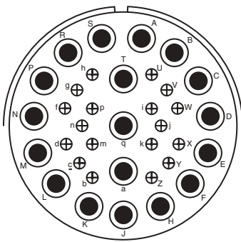
Insert Arrangement 44-53 Service Rating A Number of Contacts 18 Contact Size 16 8 (Coax) RG-124/U
