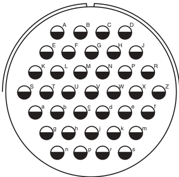
Insert Arrangement 48-53 Service Rating D Number of Contacts 37 Contact Size 12
