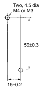
Mounting Holes
