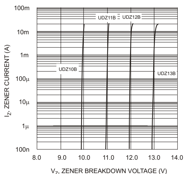
Fig. 4 Typical Reverse Characteristics, UDZ10B - UDZ13B
