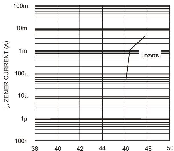
V_Z , ZENER BREAKDOWN VOLTAGE (V) Fig. 7 Typical Reverse Characteristics, UDZ47B
