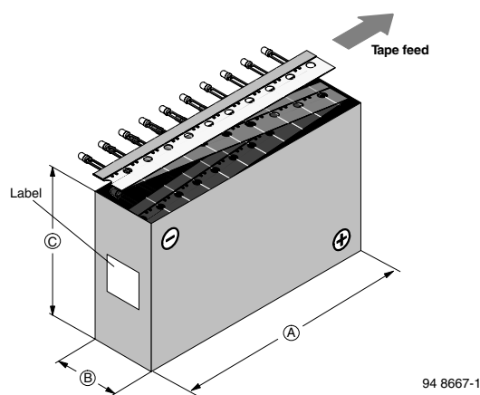
Figure 41. Tape Direction
