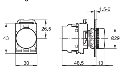
Pilot light
