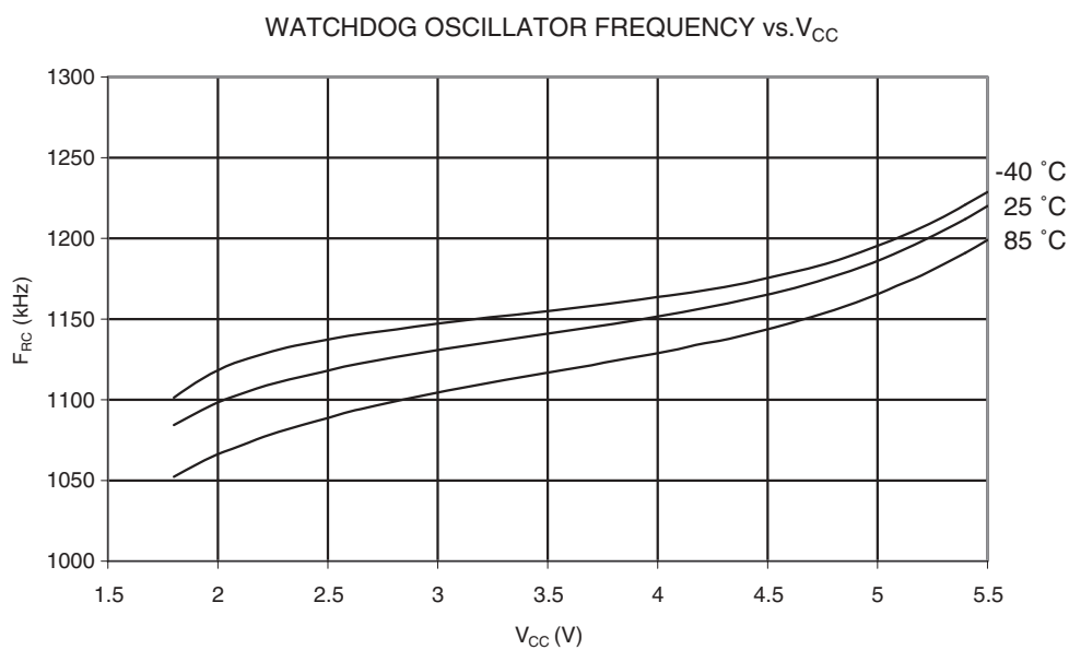
Figure 30-45. Watchdog Oscillator Frequency vs. V_{CC}
