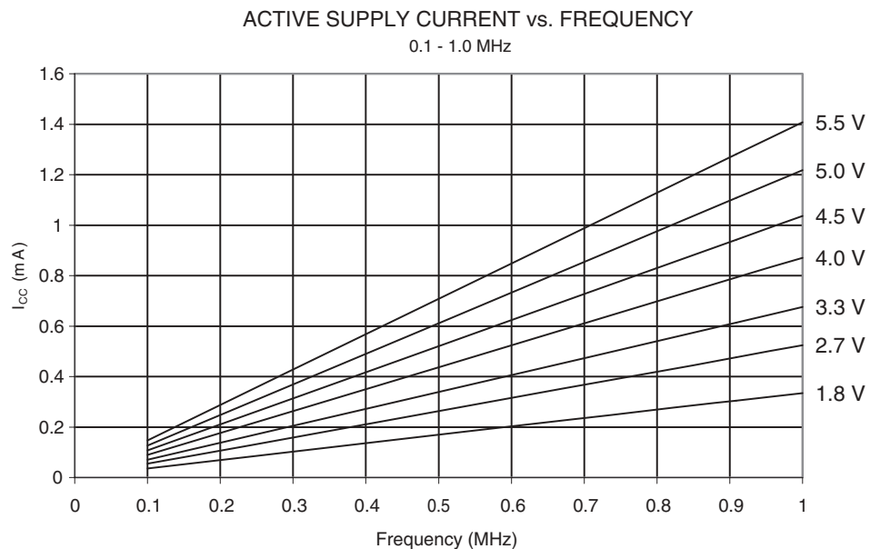
Figure 30-1. Active Supply Current vs. Frequency (0.1 - 1.0 MHz)
