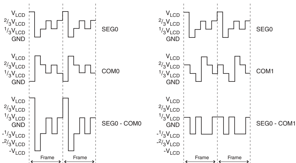
Figure 24-5. Driving a LCD with Three Common Terminals
