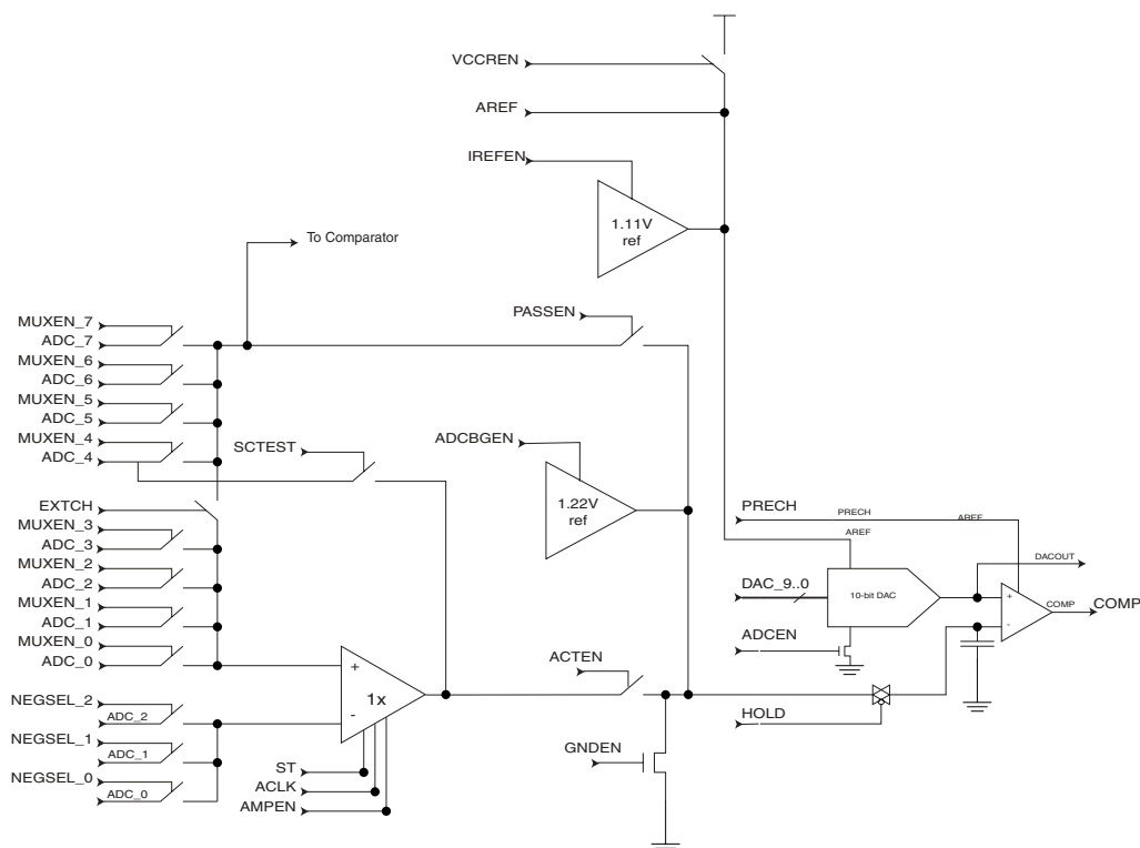
Figure 26-9. Analog to Digital Converter
