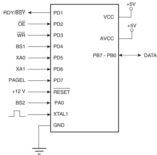
Figure 28-1. Parallel Programming
