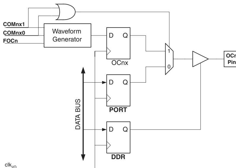
Figure 15-4. Compare Match Output Unit, Schematic
