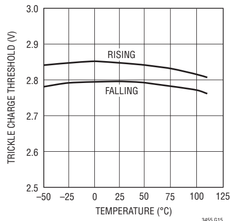
Battery Charger Trickle-Charge Threshold
