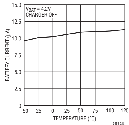
Battery Current When USB- or Wall-Powered
