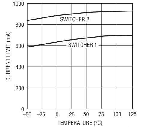
Switching Regulator Current Limit
