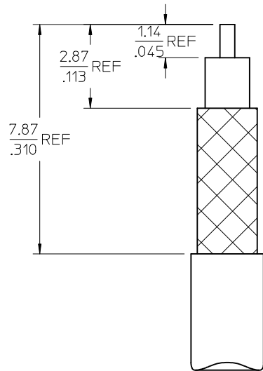
CABLE STRIP DIMENSIONS
