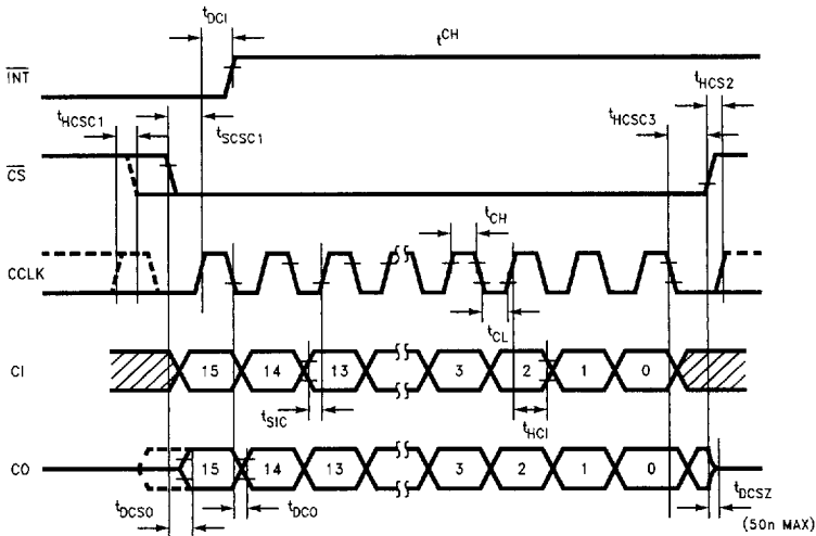
FIGURE 14a. TP3410 Enhanced MICROWIRE Control Port Timing
