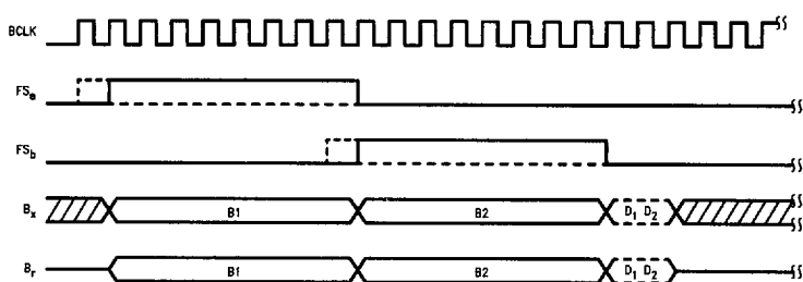
FIGURE 3-4. DSI Format 1: Master Mode
