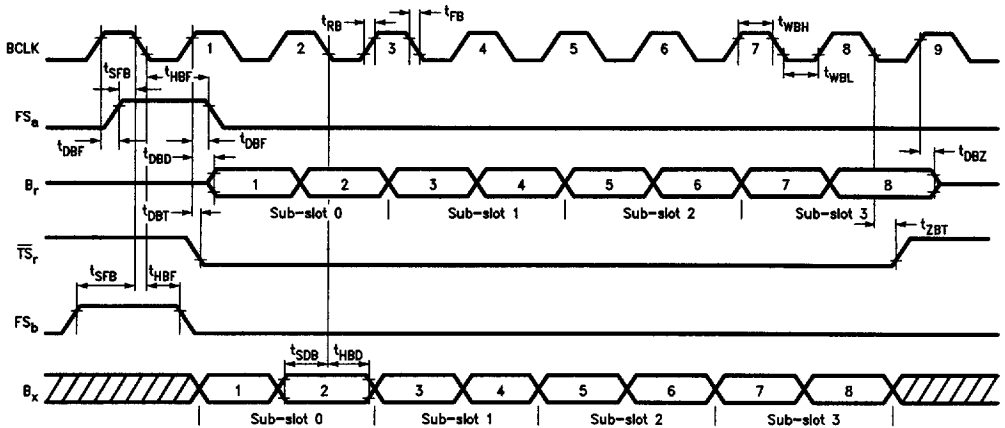
FIGURE 12. Delayed Data Timing Mode (Formats 1, 2 and 3) (Shown with TS0 Selected)
