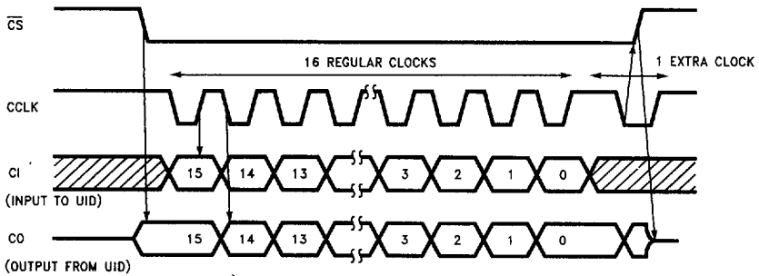
FIGURE 14c. TP3410 Alternate MICROWIRE CLOCK Format
