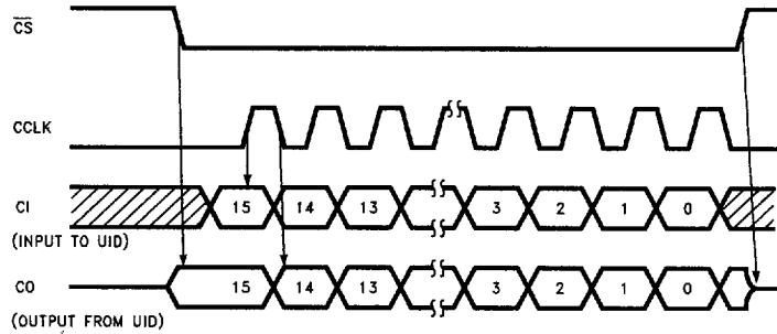
FIGURE 14b. TP3410 Normal MICROWIRE CLOCK Format
