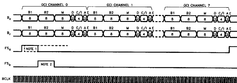
FIGURE 7. GCI Frame Structure is an Example of Multiplex Mode with BCLK = 4.096 MHz
