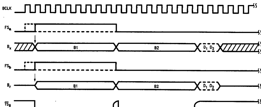
FIGURE 3-1. DSI Format 1: Slave Mode
