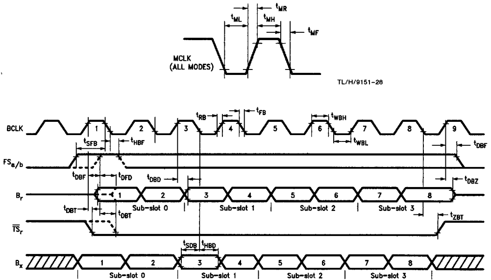
FIGURE 11. Non-Delayed Data Timing Mode (Formats 1 and 3)
