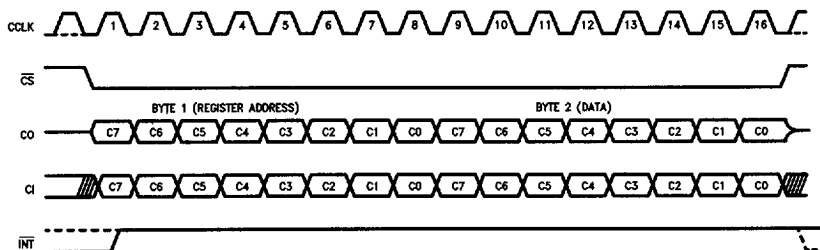
FIGURE 6. Microwire Control Port Timing: MW = 1
