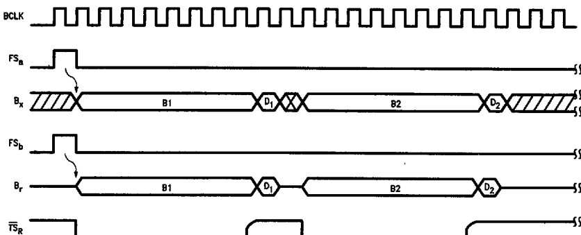
FIGURE 3-2. DSI Format 2 (IDL): Slave Mode
