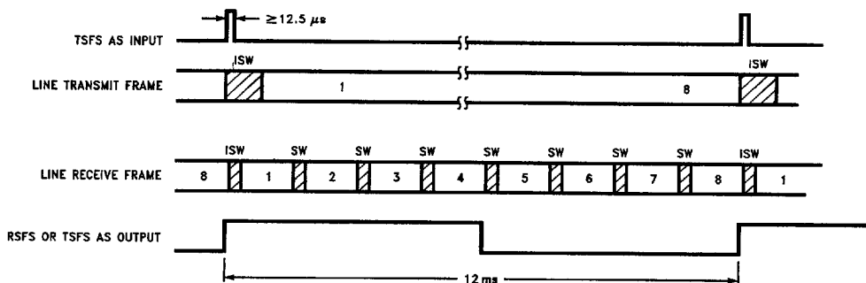
FIGURE 2. Superframe Sync Pin Timing
