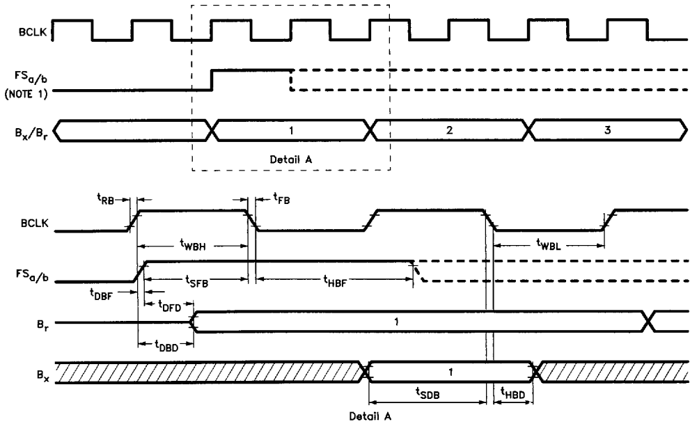
FIGURE 13. GCI and Format 4 Timing
