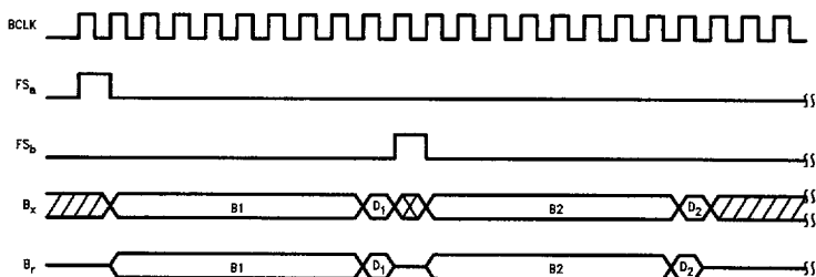
FIGURE 3-5. DSI Format 2 (IDL): Master Mode
