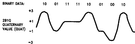
FIGURE 1. 2B1Q Line-Coding Rule
