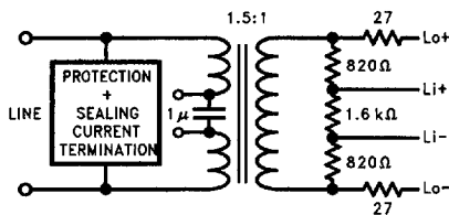
FIGURE 9. Typical Application in Microwire Mode
