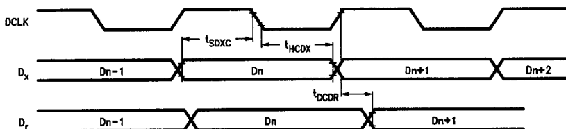
FIGURE 4. D-Port Interface Timing Using DCLK in 16 kHz Mode
