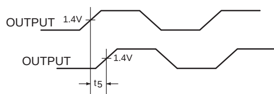
Input-Output Propagation Delay
