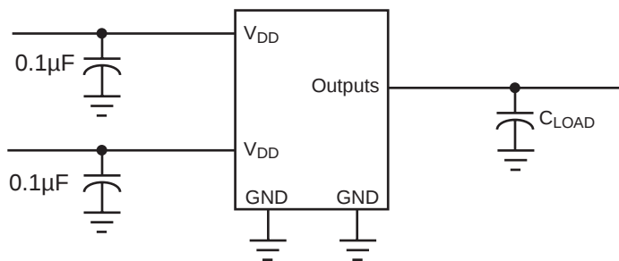
Test Circuit for all parameters except t_8
