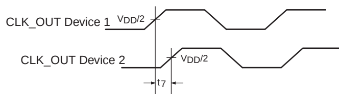
Device-Device Skew
