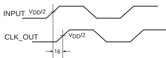
Input-Output Propagation Delay
