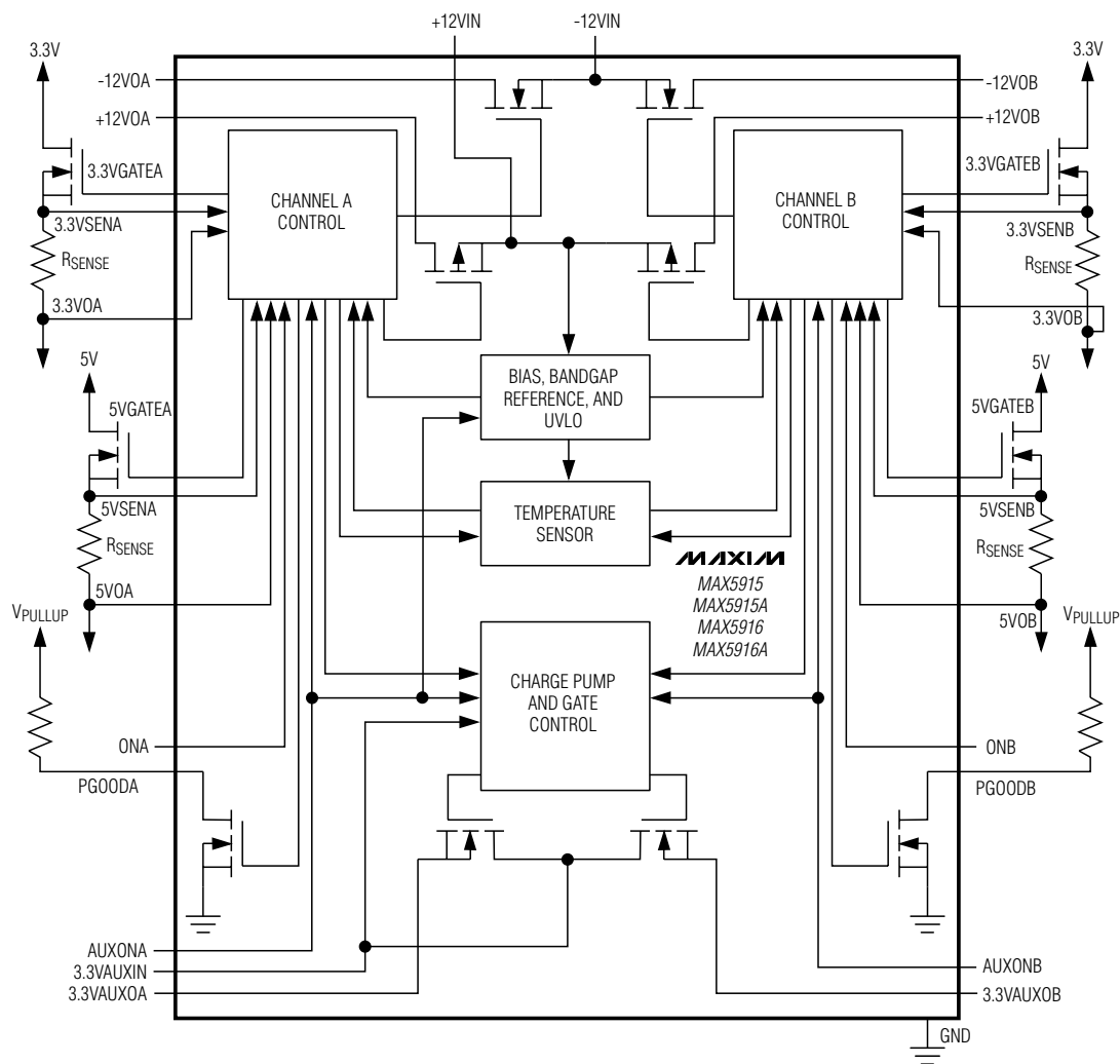
Functional Diagram
