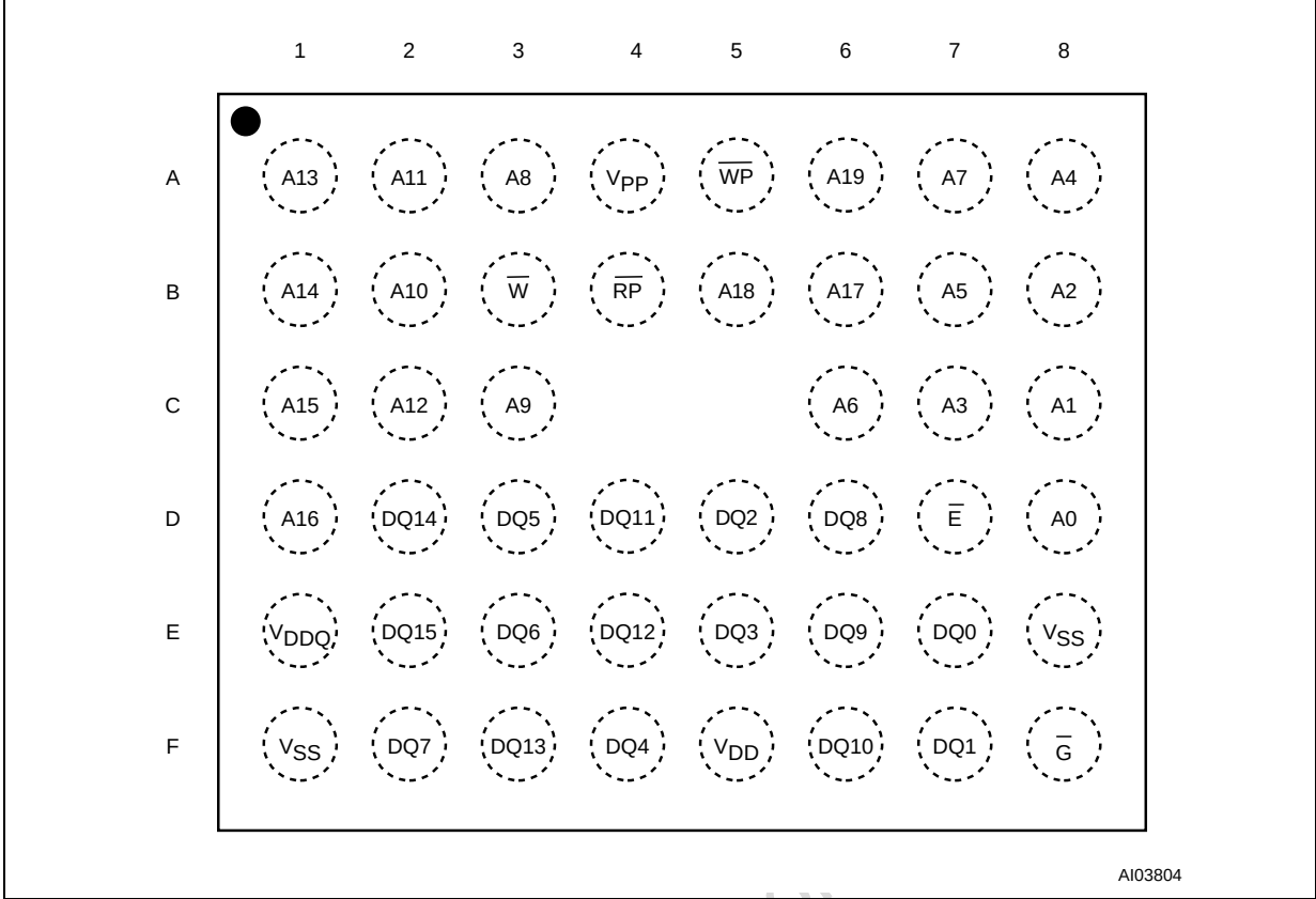
Figure 5. TFBGA Connections (Top view through package)
