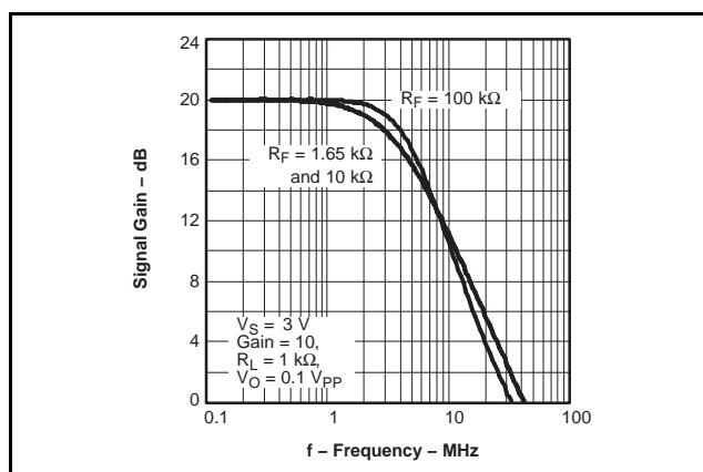
Figure 69. Signal Gain vs Frequency, V_S = 3\text{ V}
