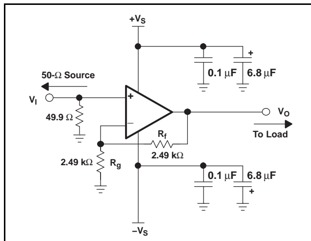
Figure 68. Wideband, Noninverting Gain Configuration
