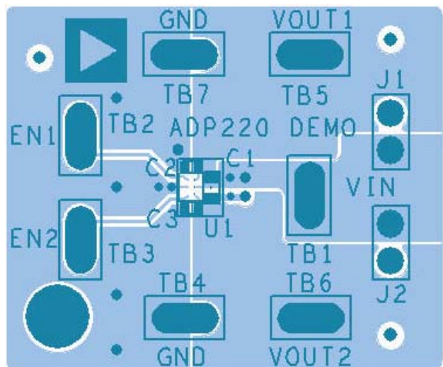
Figure 1. ADP220/ADP221 Evaluation Board
