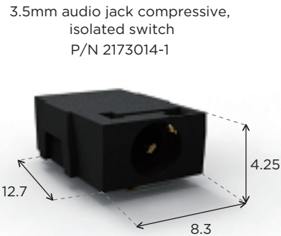
Chamfered design (10°) matches with most phone designs
