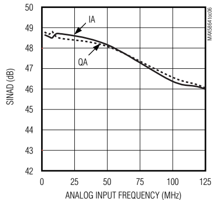
ADC SIGNAL-TO-NOISE AND DISTORTION RATIO vs. ANALOG INPUT FREQUENCY
