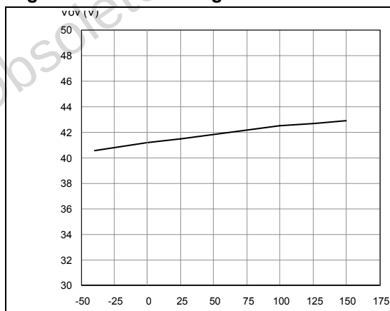
Figure 11. Over-voltage shutdown
