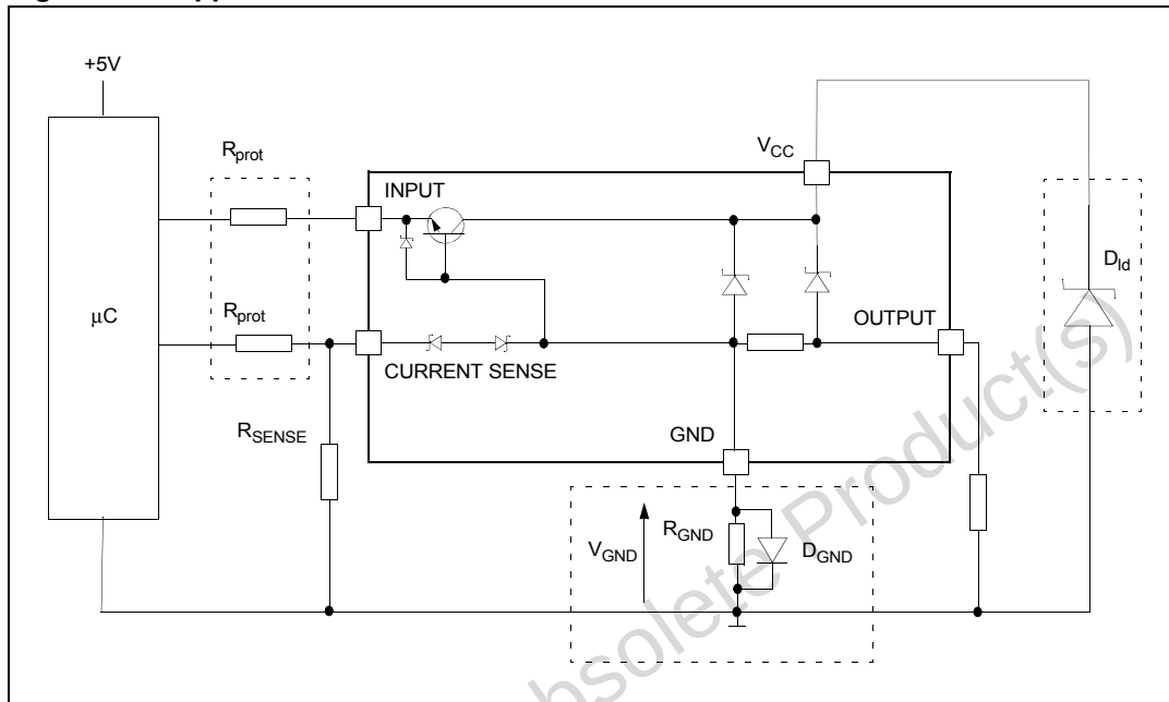
Figure 19. Application schematic
