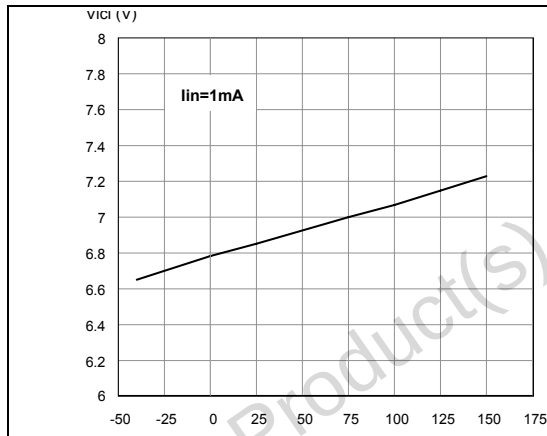
Figure 9. Input clamp voltage
