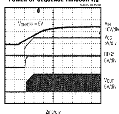
POWER-UP SEQUENCE THROUGH V_{IN}
