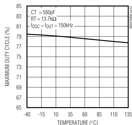
MAX15005 MAXIMUM DUTY CYCLE vs. TEMPERATURE
