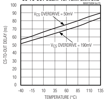
CS-TO-OUT DELAY vs. TEMPERATURE
