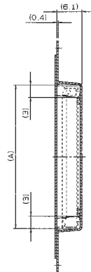
SECT. E-E
