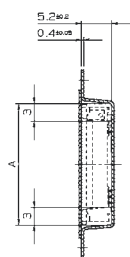
SECT. E-E
