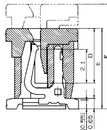
SECT. X-X
