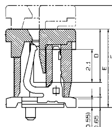
SECT. X-X
