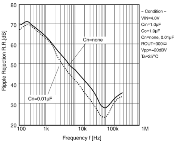
Figure 8. Ripple Rejection vs. Frequency
