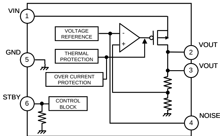
Figure 2. Block diagram
