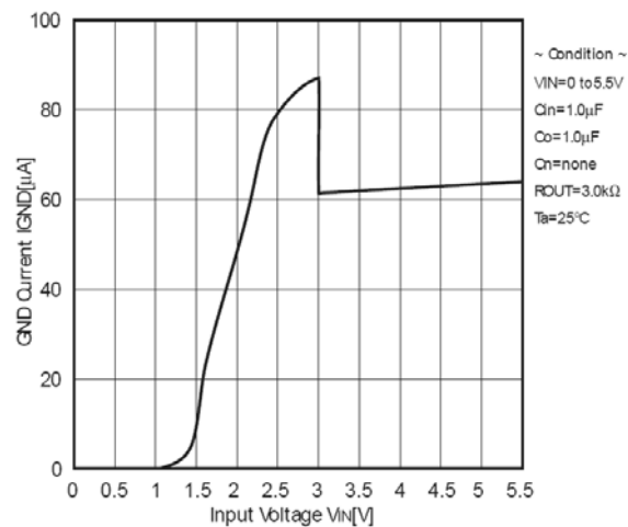
Figure 4. GND Current vs. Input Voltage
