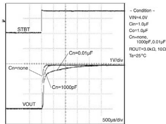
Figure 10. Startup time
