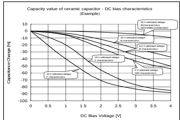
Figure 11. Capacity-bias characteristics
