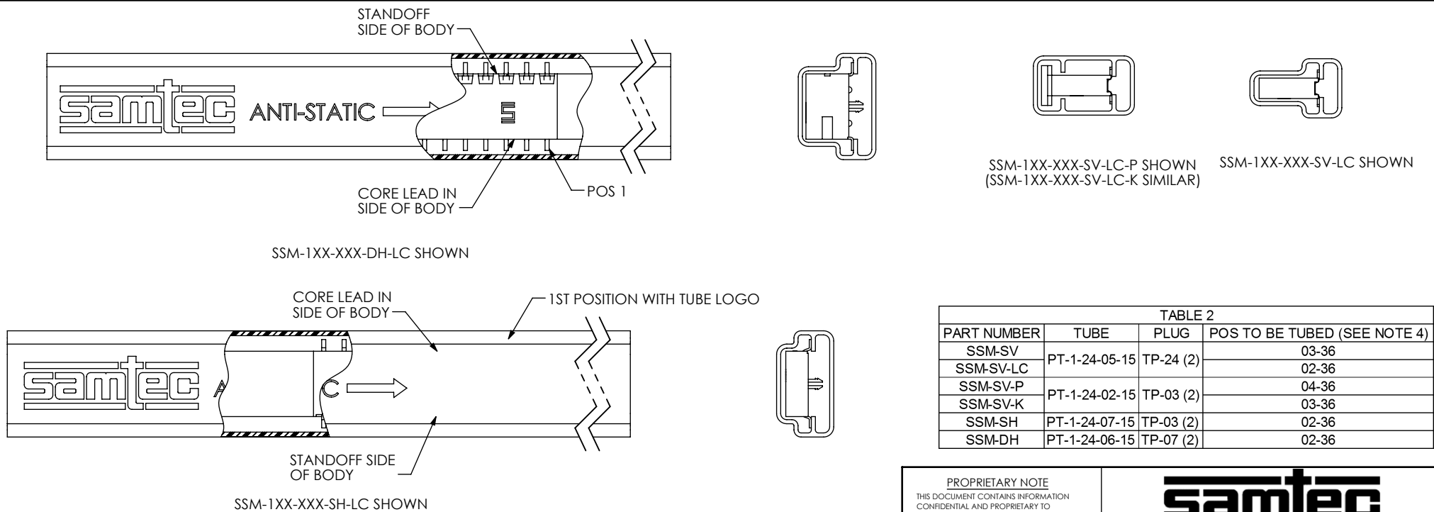
FIG 9 TUBE VIEWS
