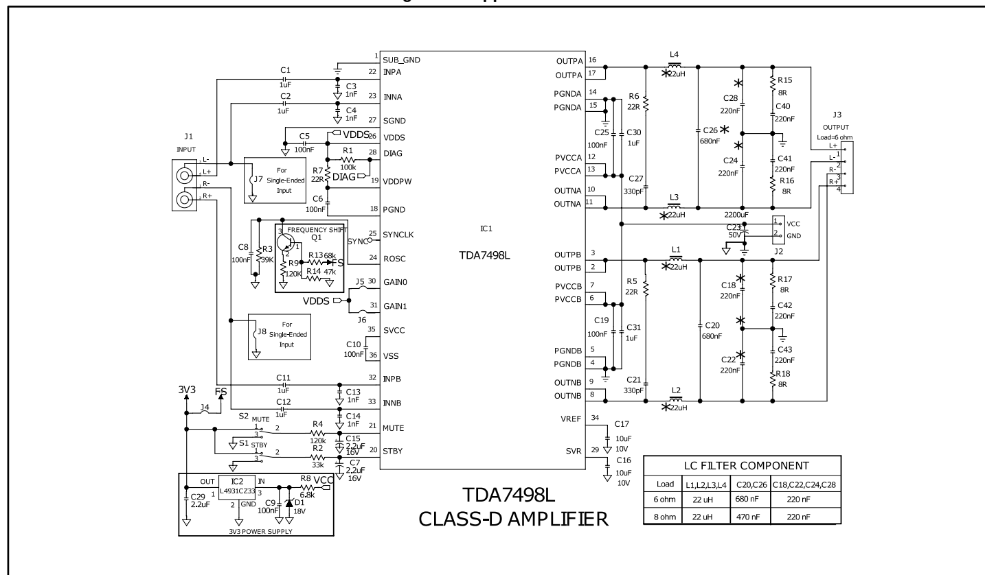
Figure 20: Application circuit
