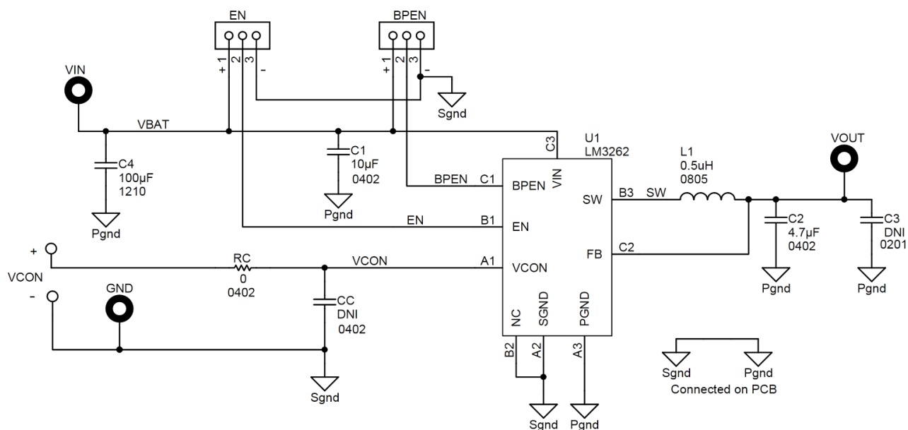
Figure 3. LM3262 Evaluation Board Schematic
