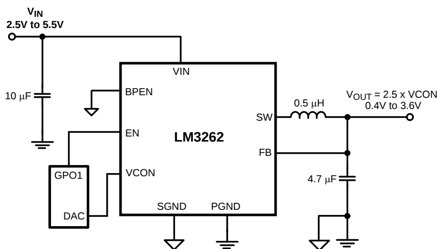
Figure 1. Application Circuit
