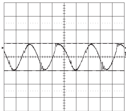
Output voltage ripple (50mV/div.) at T_{Pcb}=+25 °C, V_{in}=53 V, I_o=3.33 A resistive load with C=10 μF tantalum and 0.1 μF ceramic capacitors. Band width=20MHz. Time scale: 1 μs / div.
