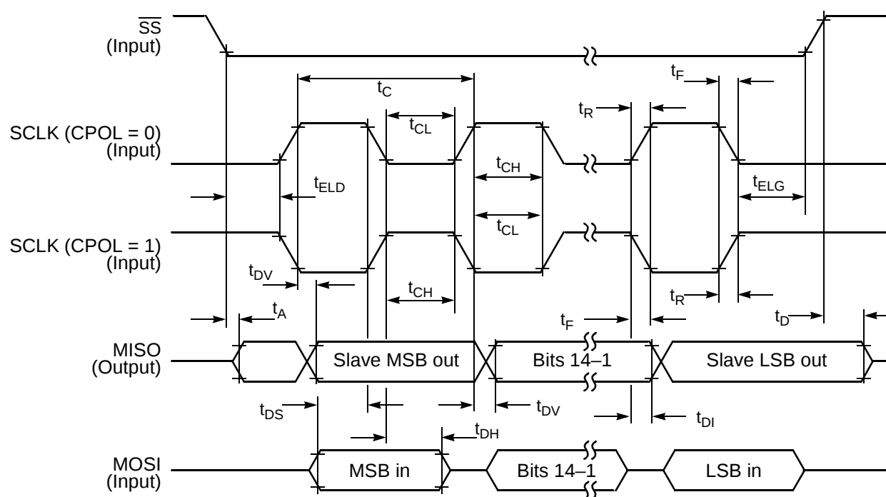
Figure 24. SPI Slave Timing (CPHA = 1)
