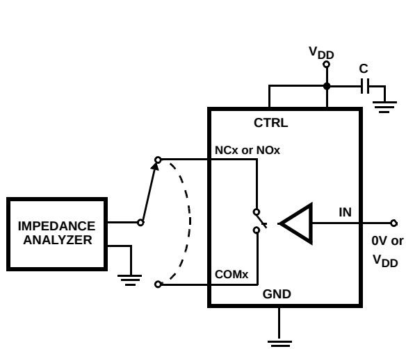
FIGURE 5. CAPACITANCE TEST CIRCUIT
