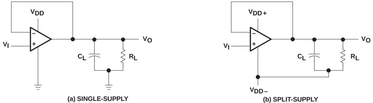
Figure 1. Unity-Gain Amplifier
