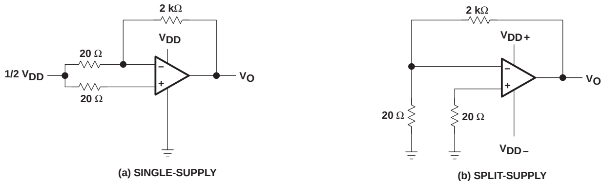
Figure 2. Noise-Test Circuit
