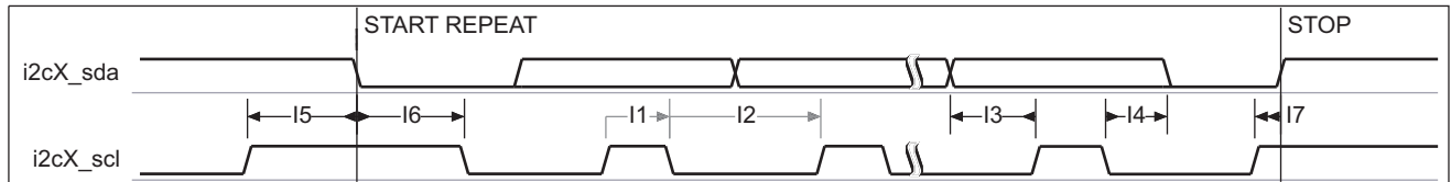
Figure 6-65. I 2 C High-Speed Mode (1) (2) (3)
