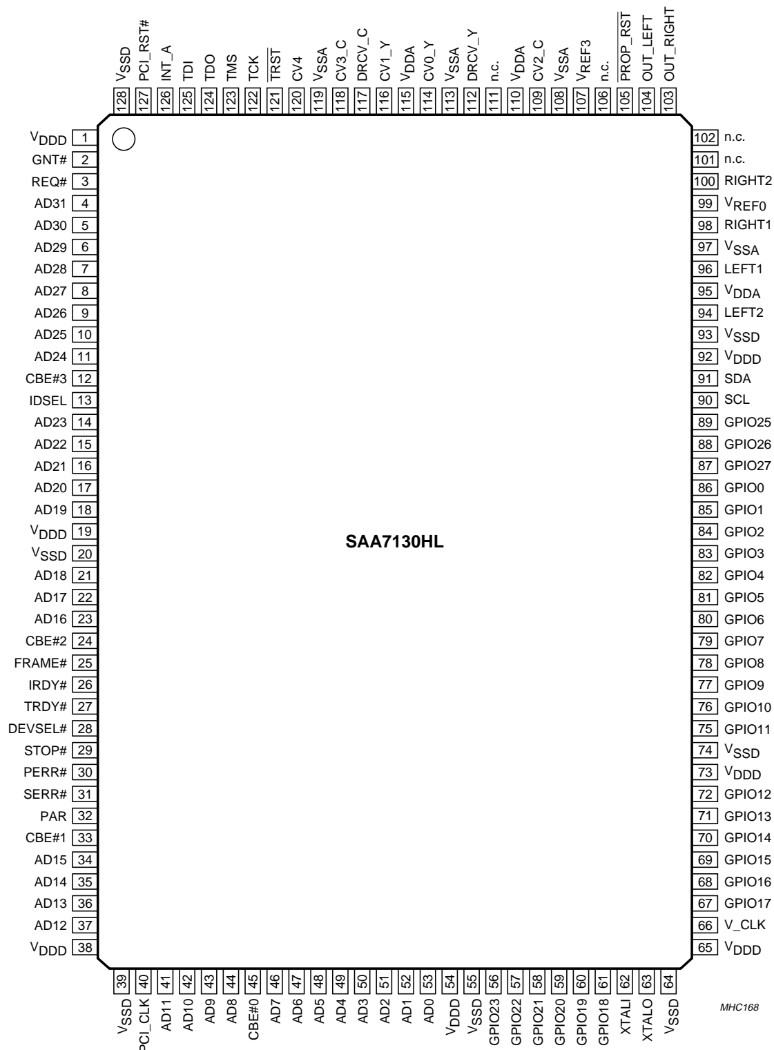
Fig.3 Pin configuration.
