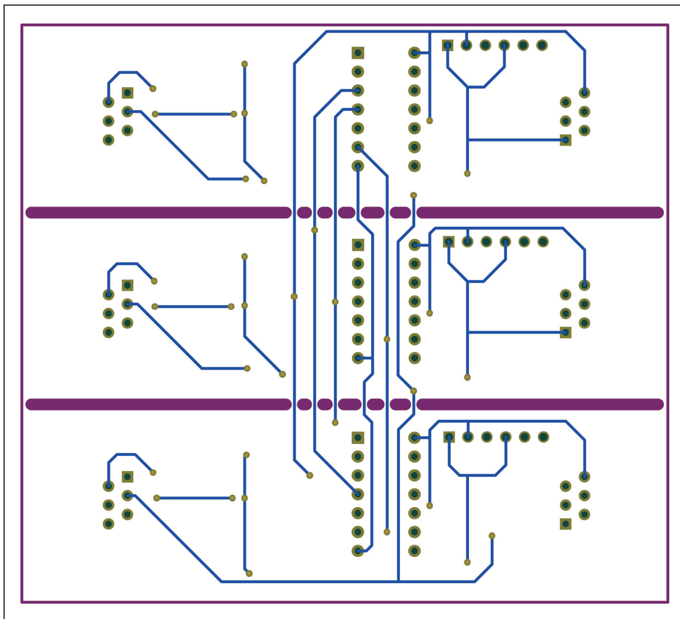
Figure 12. EV Board Layout Bottom
