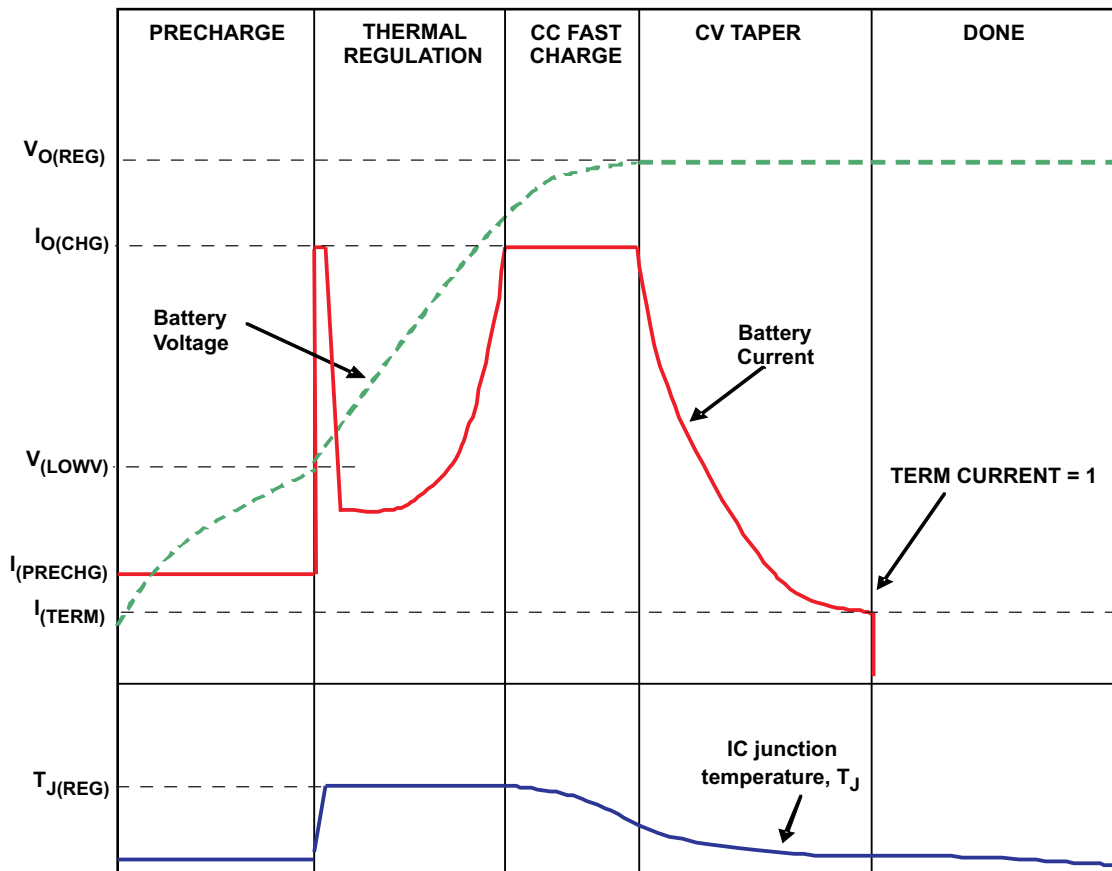
Figure 29. Thermal Loop
