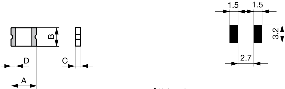
Soldering pads
