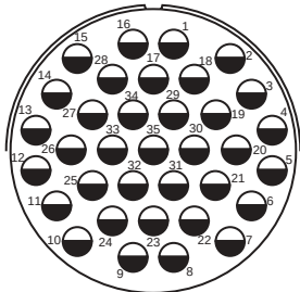
Insert Arrangement 40-35 Service Rating D Number of Contacts 35 Contact Size 12
