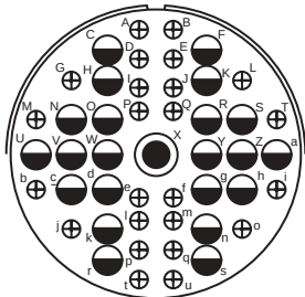
Insert Arrangement 40-9 Service Rating A Number of Contacts 1 22 24 Contact Size 8 12 16
