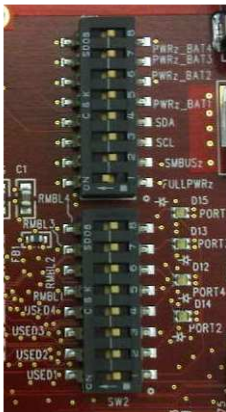
Figure 2. Configuration Switches
