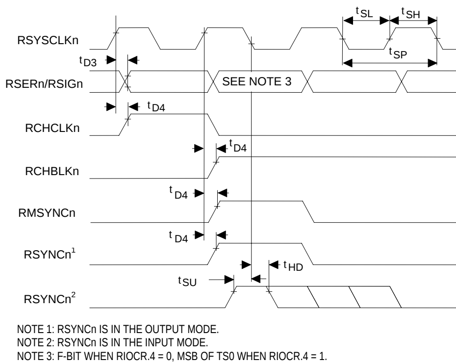
Figure 13-8. Receive Framer Timing—Line Side
