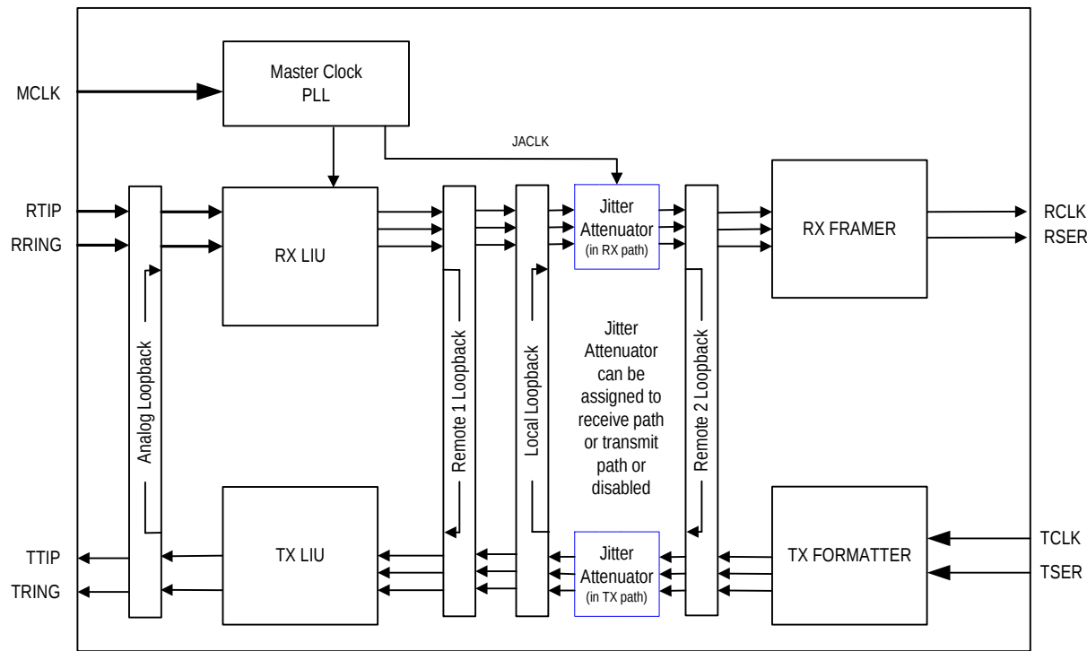
Figure 9-27. Loopback Diagram
