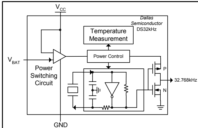
Figure 3. Block Diagram
