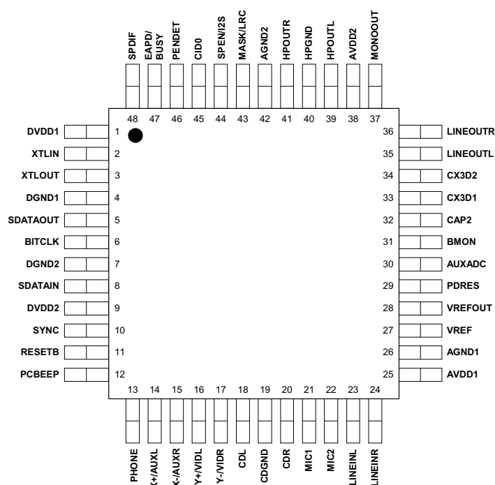
Figure 1 TQFP Pinout
