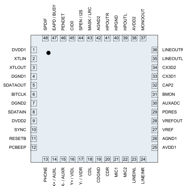
Figure 2 QFN Pinout
