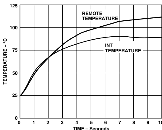
Figure 11. Response to Thermal Shock
