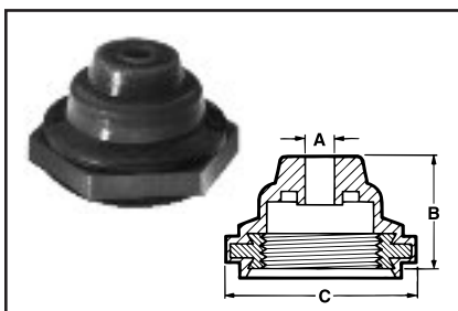
Half-Toggle Boots (toggle actuator protrudes) – IP66/68 Rated Figure 3
