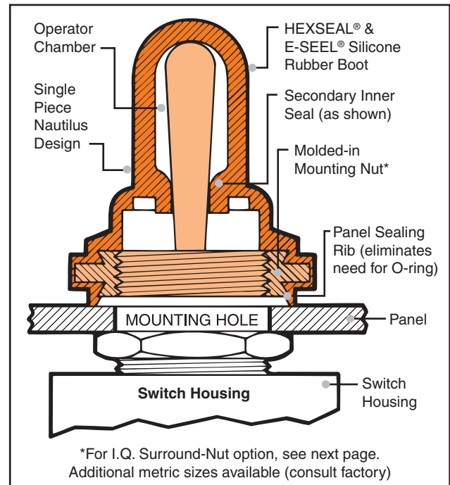
FIGURE 1 Full-Toggle Boot with Integral Secondary Inner Seal – IP66/68 Rated Figure 1
