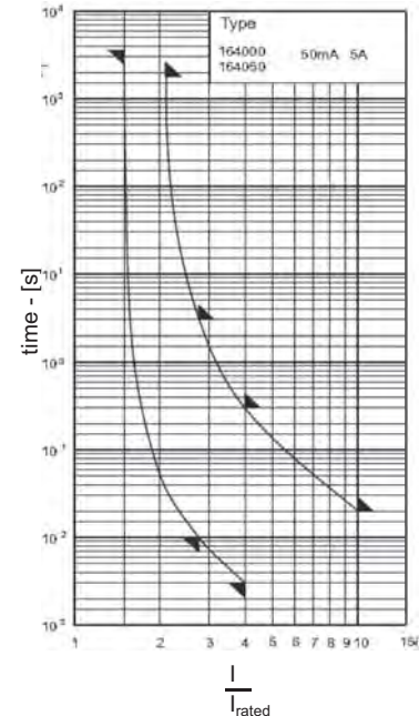
Time-Current Characteristics
