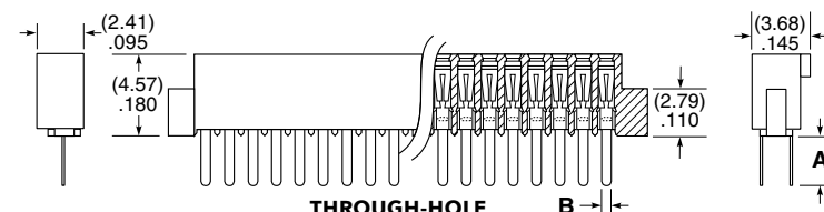
THROUGH-HOLE
