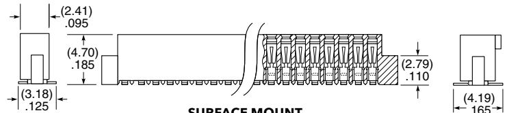
SURFACE MOUNT
