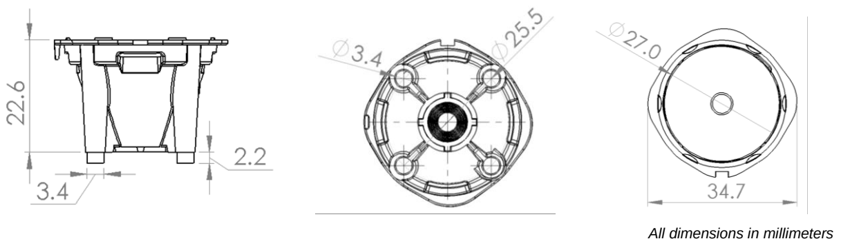
Figure 2. Layout features and dimensions of the lens assembly (lens in a holder)
