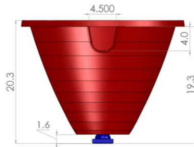
Lens: Side view showing lens gate
